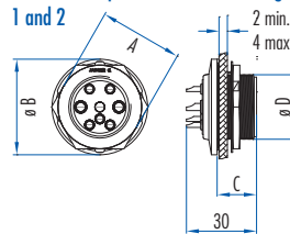
Circular male panel connectors housings 1 and 2
