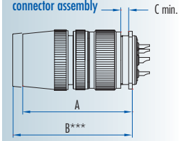
Square panel connector / Cable connector assembly
