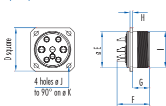
Square panel connector
