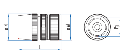
Cable connector
