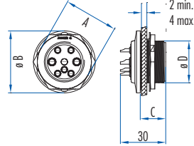
Coupler connector
