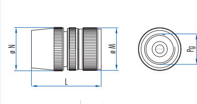
Coupler connector
